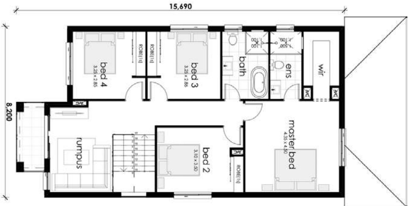
First Floor
