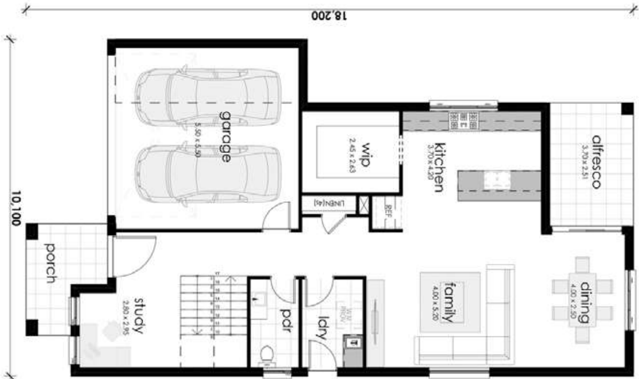
Ground Floor
